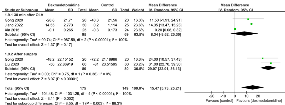
Supplementary Fig. 7. Forest plot diagram showing SOD levels. SD: standard deviation, IV: inverse variance, SOD: superoxide dismutase, OLV: one-lung ventilation.
