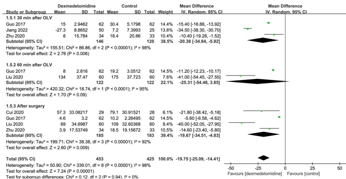
Supplementary Fig. 3. Forest plot diagram of TNF- \alpha levels. SD: standard deviation, IV: inverse variance, OLV: one-lung ventilation.
